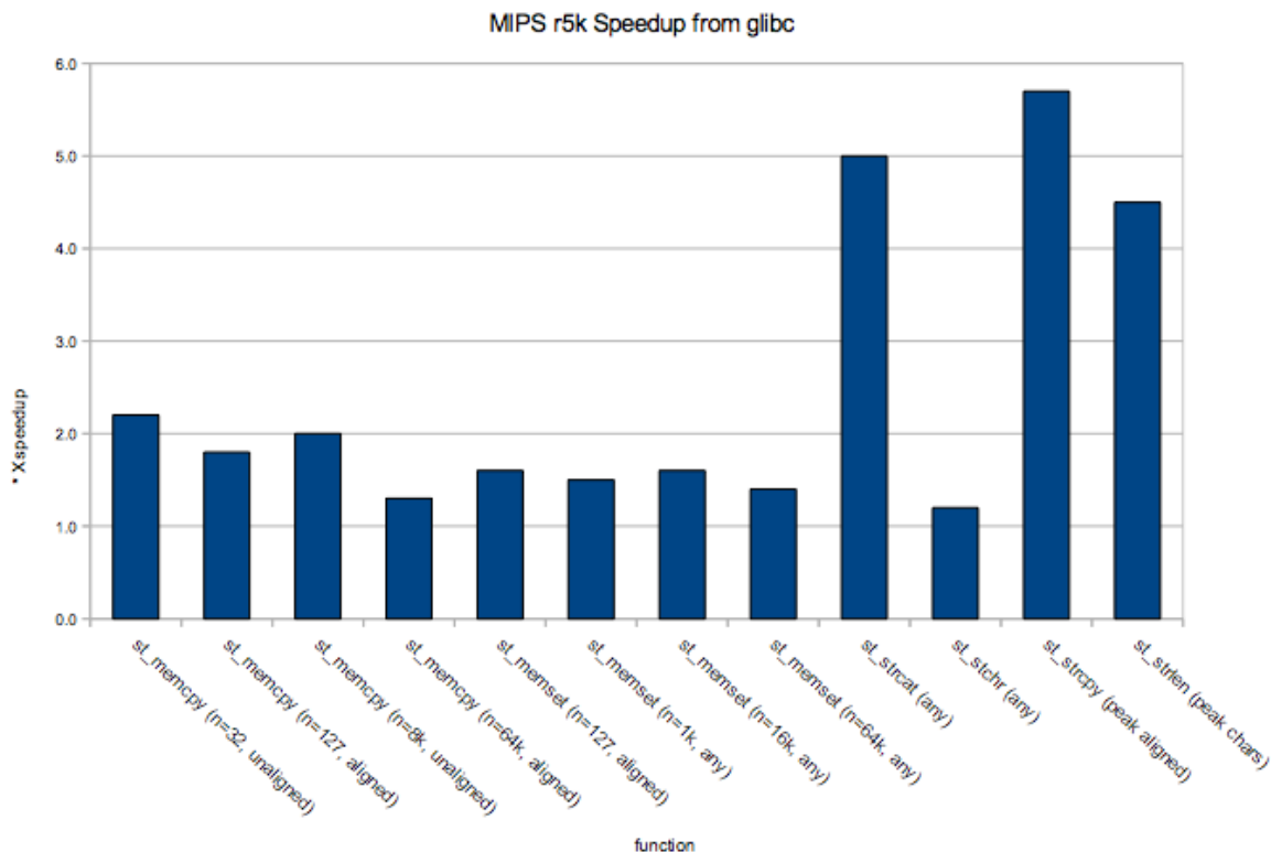
Speedups of string and memory functions over GNU
