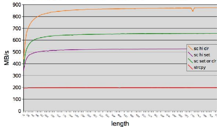
Performance versus GNU strcpy
