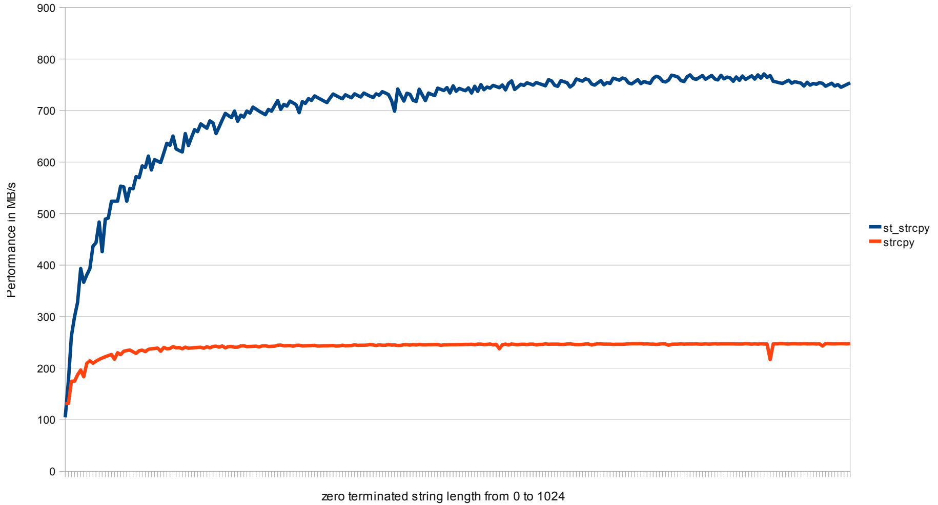
Scalar optimized st_strcpy performance
